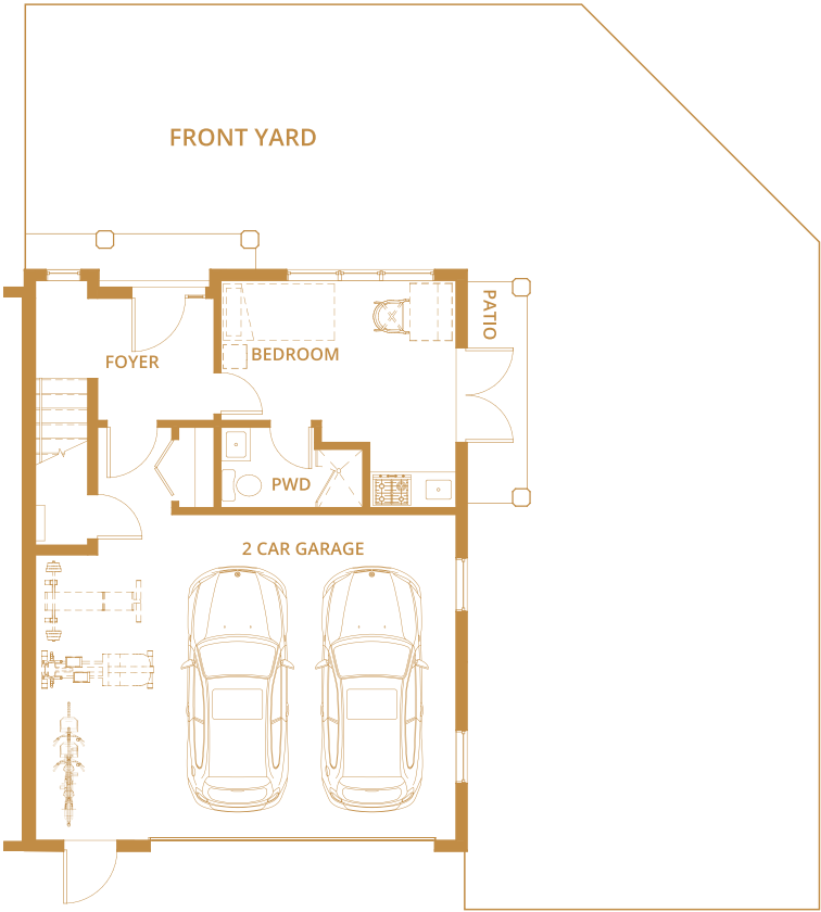
GROUND FLOOR: 345 SQ. FT.
