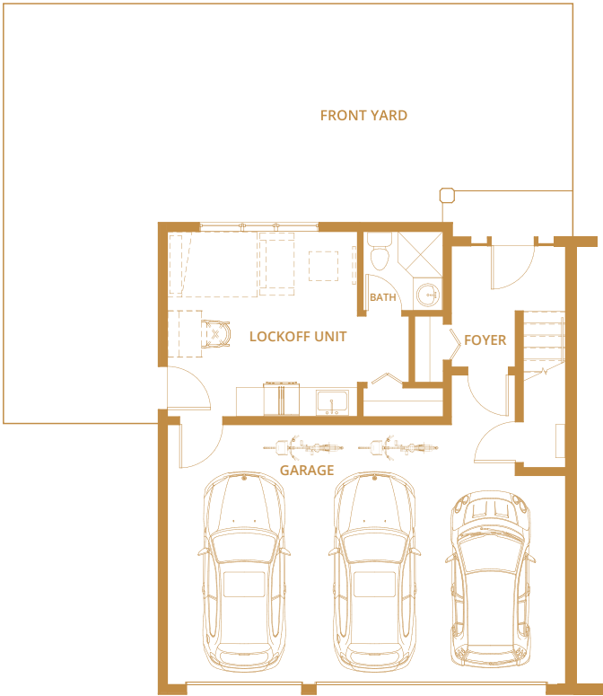
GROUND FLOOR: 425 SQ. FT.
